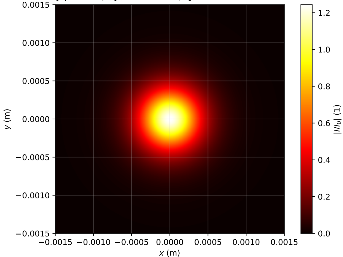
Intensity profile I(x, y, z = 2.388m)/I_0 , P_{in}=0.8P_{cr} , artificial time
